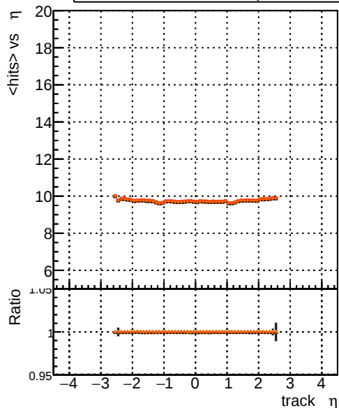
mean hits vs \eta — Iter1-Patatrack+CleanedTriplets-LSTBuild_Iter2-LSTSeed-CKFitBuild-CKFit — Iter1-Patatrack+CleanedTriplets-LSTBuild_Iter2-LSTSeed-MkFitBuild-CKFit — Iter1-Patatrack+CleanedTriplets-LSTBuild_Iter2-LSTSeed-MkFitBuild-MkFitFit
