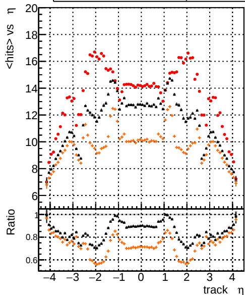
mean hits vs \eta — Iter1-Patatrack+CleanedTriplets-LSTBuild_Iter2-LSTSeed-CKFFit — Iter1-Patatrack+CleanedTriplets-LSTBuild_Iter2-LSTSeed-MkFitBuild-CKFFit — Iter1-Patatrack+CleanedTriplets-LSTBuild_Iter2-LSTSeed-MkFitBuild-MkFitFit
