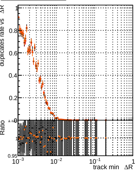
Legend: - \bullet DQM AlpakaBaselineSeedMaskingLSTSeeding HARVESTING - \bullet DQM AlpakaBaselineSeedMaskingLSTSeeding mkFit HARVESTING - \bullet DQM AlpakaBaselineSeedMaskingLSTSeeding mkFitFIT HARVESTING
