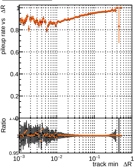
Legend: - \bullet DQM AlpakaBaselineSeedMaskingLSTSeeding HARVESTING - \bullet DQM AlpakaBaselineSeedMaskingLSTSeeding mkFit HARVESTING - \bullet DQM AlpakaBaselineSeedMaskingLSTSeeding mkFitFIT HARVESTING
