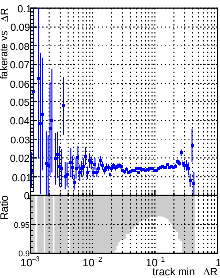
Fake rate vs \Delta R(\text{track}, \text{jet}) DQM_base_HARVESTING
