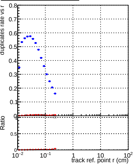
—■— /ceph/cms/store/user/legianni/filesDQMHLT_wLST/AlpakaBaselineSeedMaskingLSTSeeding/DQM_base_HARVESTING —●— /ceph/cms/store/user/legianni/filesDQMHLT_wLST/AlpakaBaselineSeedMaskingLSTSeeding/DQM_AlpakaBaselineSeedM
