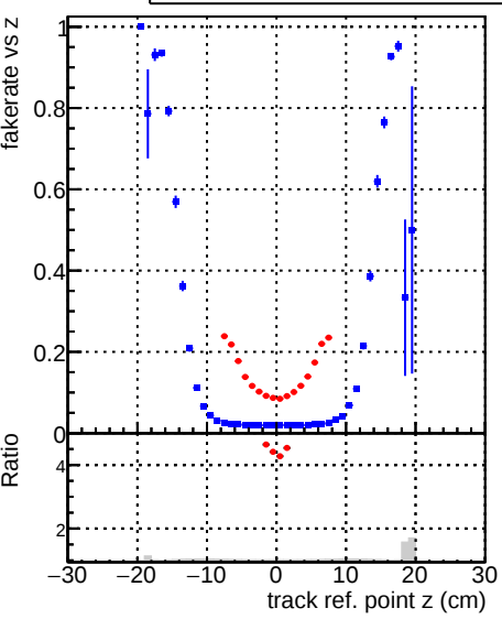
—■— /ceph/cms/store/user/legianni/filesDQMHLT_wLST/AlpakaBaselineSeedMaskingLSTSeeding/DQM_base_HARVESTING —●— /ceph/cms/store/user/legianni/filesDQMHLT_wLST/AlpakaBaselineSeedMaskingLSTSeeding/DQM_AlpakaBaselineSeedM
