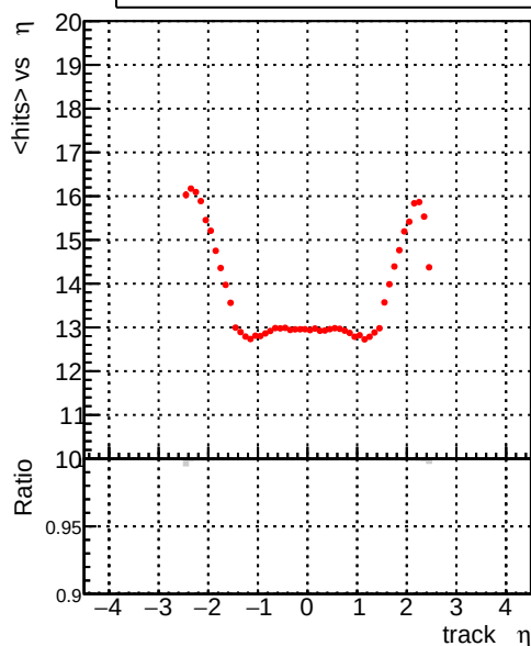
mean hits vs \eta /ceph/cms/store/user/legianni/filesDQMHLT_wLST/AlpakaBaselineSeedMaskingLSTSeeding/DQM_AlpakaBaselineSeed
