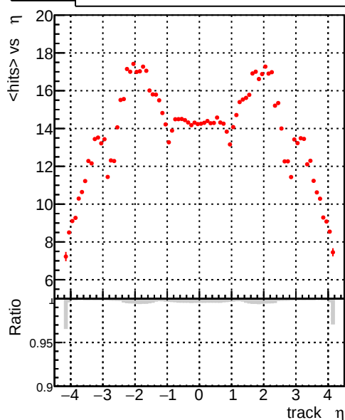
mean hits vs \eta /ceph/cms/store/user/legianni/filesDQMHLT_wLST/AlpakaBaselineSeedMaskingLSTSeeding/DQM_AlpakaBaselineSeedMaskingLSTSeeding
