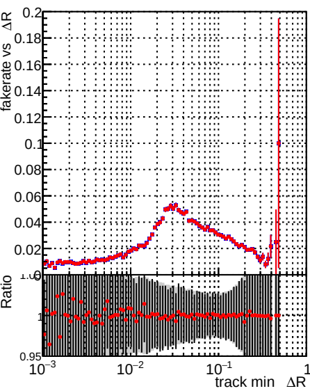
Fake rate vs \Delta R (track, jet) DQM_harvest_CKF_CKF DQM_harvest_mkFit_CKF
