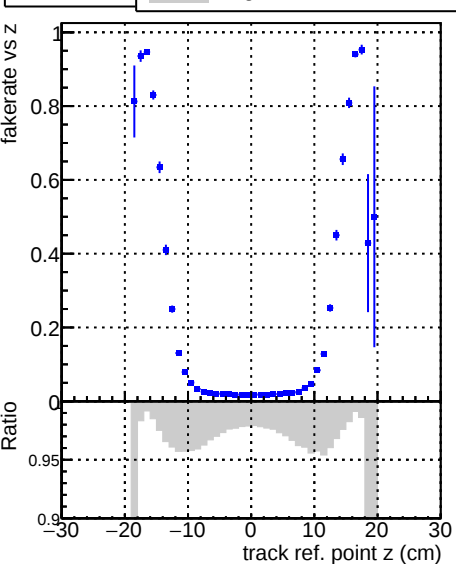
Fake rate vs v DQM_harvest_mkFit_CKF_keep
