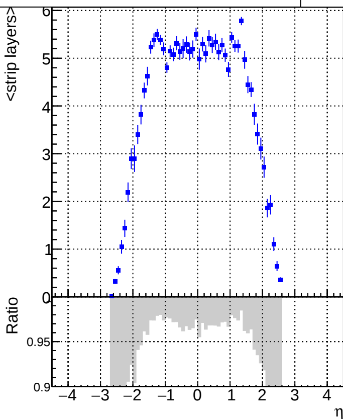
DQM_V0001_R000000001_Global_CMSSW_X_Y_Z_RECO
