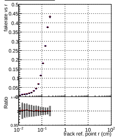
—•— DQM_harvest_CKF_keep —•— DQM_harvest_mkFit_CKF_keep —•— DQM_harvest_mkFit_CKF_keep TESTNOFIT
