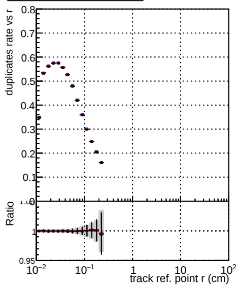
—•— DQM_harvest_CKF_keep —•— DQM_harvest_mkFit_CKF_keep —•— DQM_harvest_mkFit_CKF_keep TESTNOFIT
