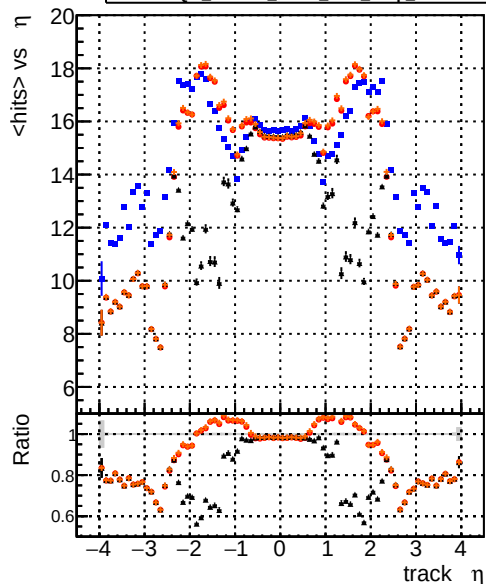
mean hits DOM_harvest_CKF_CKF_keep DOM_harvest_mkFit_CKF_keep DOM_harvest_mkFit_CKF_keep_TESTNOFIT DOM_harvest_mkFit_CKF_keep_TESTFIT
