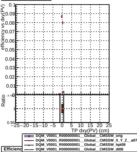
Efficiency vs Dxy(PV)
