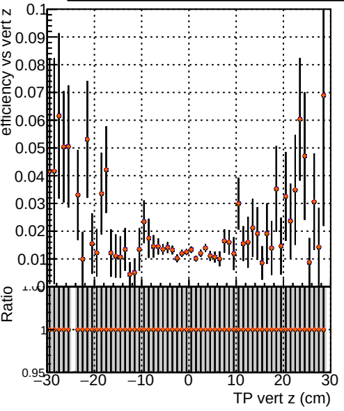
Efficiency vs vertpos —●— DQM_V0001_R000000001 Global CMSSW_orig —●— DQM_V0001_R000000001 Global CMSSW_X_Y_Z_all7 —●— DQM_V0001_R000000001 Global CMSSW_hpt08 —●— DQM_V0001_R000000001 Global CMSSW_dt08
