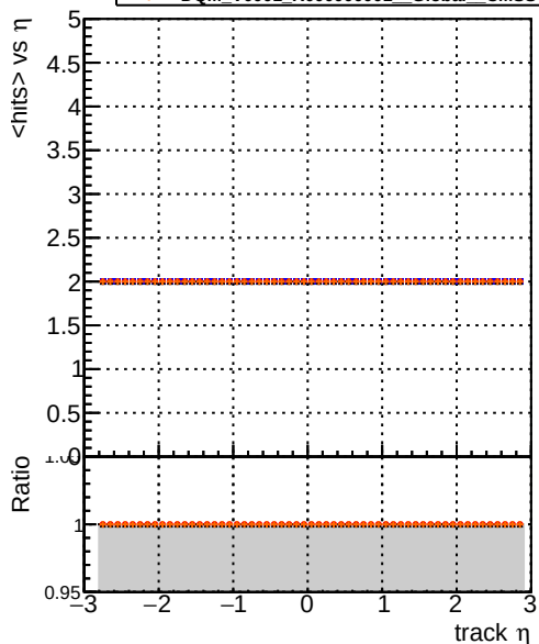
mean hits vs \eta DQM_V0001_R000000001_Global_CMSSW_orig DQM_V0001_R000000001_Global_CMSSW_X_Y_Z_all7 DQM_V0001_R000000001_Global_CMSSW_hpt08 DQM_V0001_R000000001_Global_CMSSW_dt08
