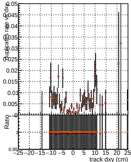
Legend for Fake rate vs d, Duplicates rate vs Dxy, and Pileup rate vs dxy: Global CMSSW orig CMSSW 0096 CMSSW 0098 all7
