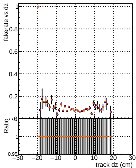
Fake rate vs d DOM V0001 B000000000001 Global CMSSW orig Global CMSSW dr08 Global CMSSW dr07 Global CMSSW dr06
