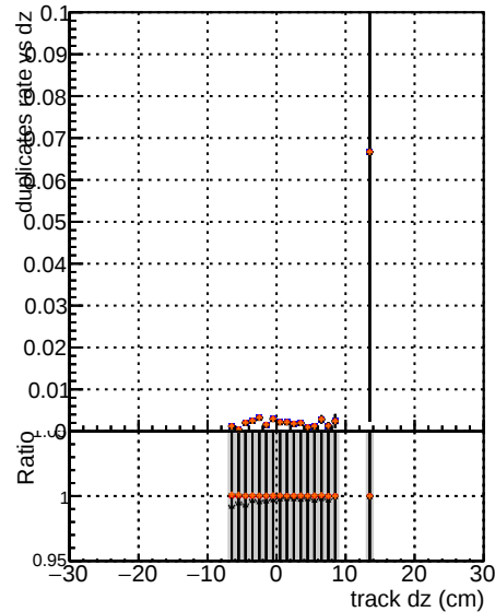
CMSSW-4_08-017
