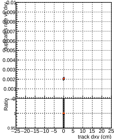
CMSSW-4_08-017
