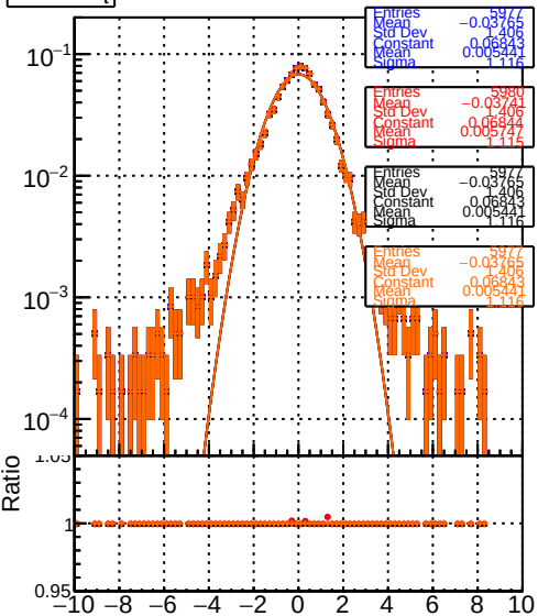
pull of p_t
