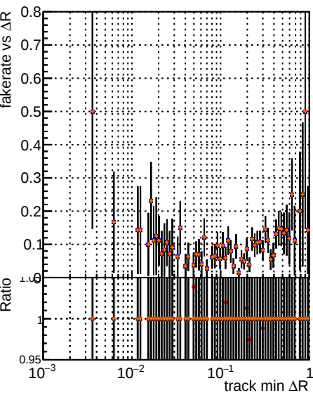
Fake rate vs \Delta R(\text{track, jet}) DQM V00001 R00000000001 Global CMSSW orig Z all7 Global CMSSW dt08
