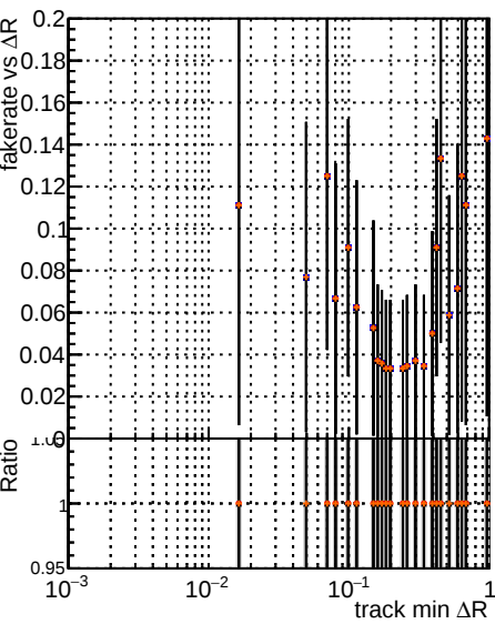
Fake rate vs \Delta R(\text{track, jet}) DQM V00001 R00000000001 Global CMSSW orig Z all7 DQM V00001 R00000000001 Global CMSSW orig Z all7 DQM V00001 R00000000001 Global CMSSW orig Z all7
