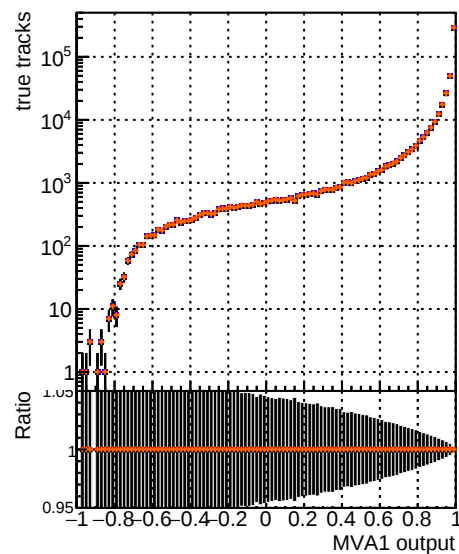
N of associated tracks (recoToSim) vs MVA1
