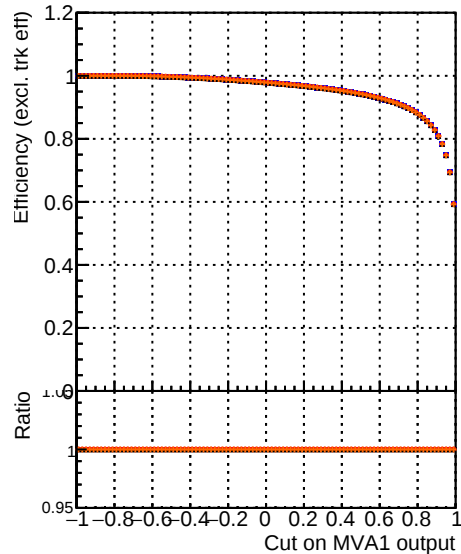
Efficiency (tracking eff factorized out) vs. MVA1
