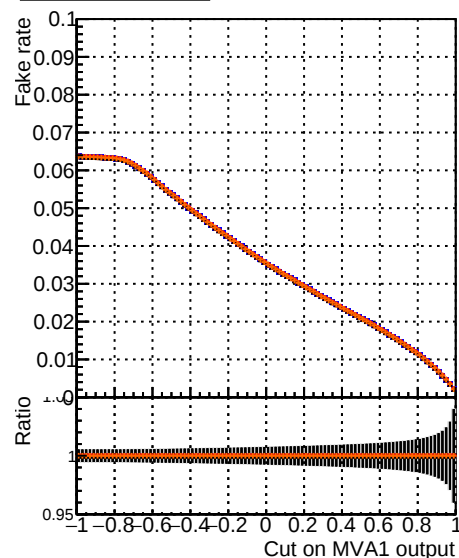
Fake rate vs. MVA1
