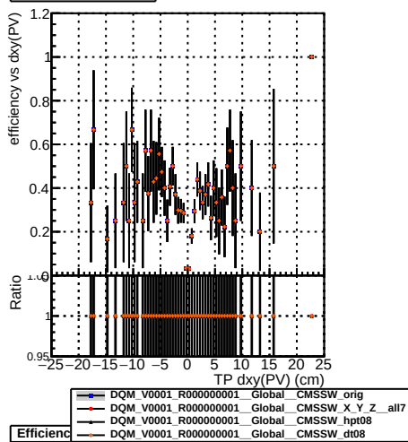
Efficiency vs Dxy(PV)
