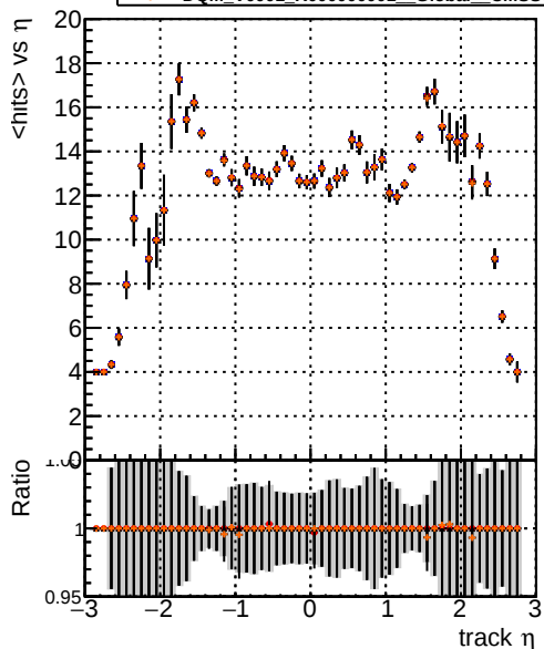
mean hits vs \eta DQM_V0001_R000000001_Global_CMSSW_Orig DQM_V0001_R000000001_Global_CMSSW_X_Y_Z_all7 DQM_V0001_R000000001_Global_CMSSW_hpt08 DQM_V0001_R000000001_Global_CMSSW_dtt08
