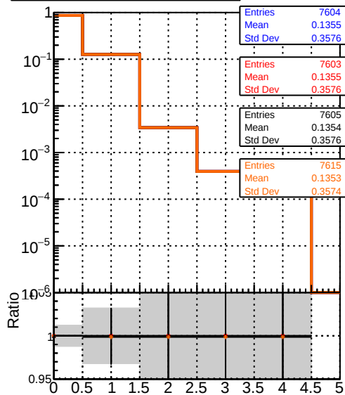
mean hits vs \eta DQM_V0001_R000000001_Global_CMSSW_Orig DQM_V0001_R000000001_Global_CMSSW_X_Y_Z_all7 DQM_V0001_R000000001_Global_CMSSW_hpt08 DQM_V0001_R000000001_Global_CMSSW_dtt08
