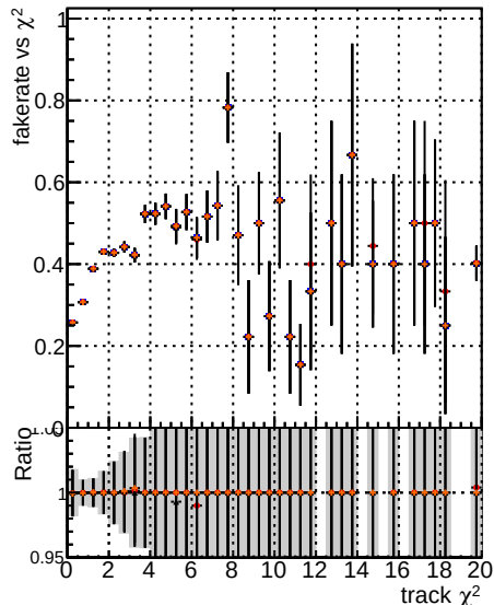
Fake rate vs. DQM_V0001 Global CMSSW_orig_Z_all7 DQM_V0001 CMSSW_0098
