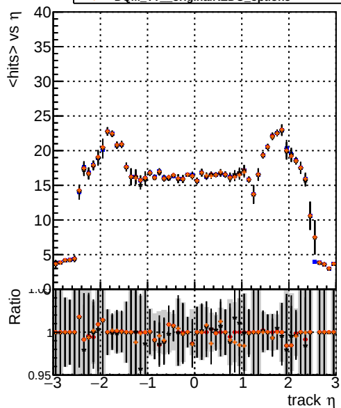
mean hits vs \eta Legend: /data2/legianni/pareto-opt/restart/CMSSW_14_0_5/src/MIV-plot/DQM_TT_original_PU (blue line), DQM_TT_originalREDO_option3 (red line with dots), DQM_TT_originalREDO_option4 (black line with dots), DQM_TT_originalREDO_option5 (orange line with dots)
