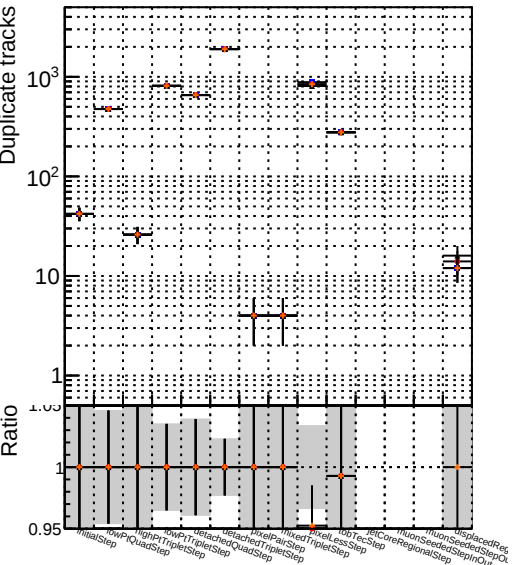
/data2/legianni/pareto-opt/restart/CMSSW_14_0_5/src/MTV-plot/DQM_TT__original_PU DQM_TT__original_PU_option3
