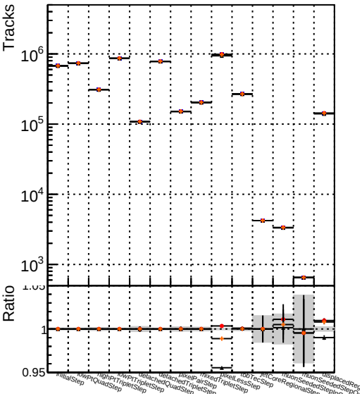
/data2/legianni/pareto-opt/restart/CMSSW_14_0_5/src/MTV-plot/DQM_TT__original_PU DQM_TT__original_PU_option3
