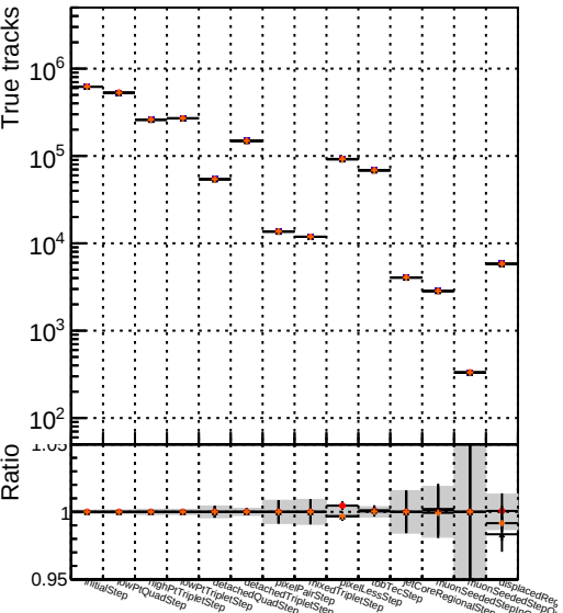
/data2/legianni/pareto-opt/restart/CMSSW_14_0_5/src/MTV-plot/DQM_TT__original_PU DQM_TT__original_PU_option3
