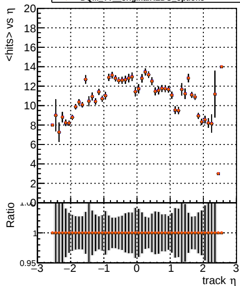
mean hits vs \eta Legend: /data2/legianni/pareto-opt/restart/CMSSW_14_0_5/src/MIV-plot/DQM_TT_original_PU (blue line), DQM_TT_originalREDO_option3 (red line), DQM_TT_originalREDO_option4 (black line), DQM_TT_originalREDO_option5 (orange line)
