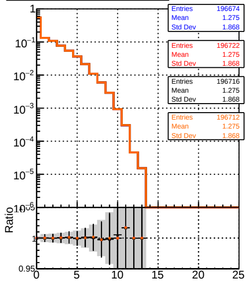
mean hits /data2/legianni/pareto-opt/restart/CMSSW_14_0_5/src/MIV-plot/DQM_TT_original_PU DQM_TT_originalREDO_option3 DQM_TT_originalREDO_option4 DQM_TT_originalREDO_option5
