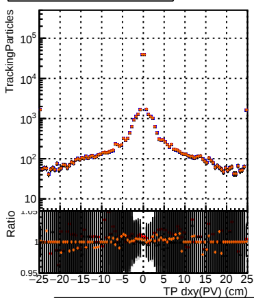
Legend for N of simulated tracks vs dxy(PV): DQM_TT_original DQM_TT_debug_bestinlayer75_epcoh10 DQM_TT_debug_truthallhits75_epcoh11 DQM_TT_debug_truthsimuptolayer75_epcoh11
