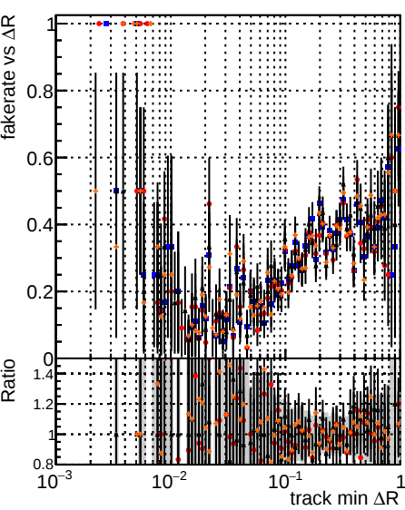
Fake rate vs \Delta R(\text{track, jet}) DQM TT original bestinlayer75 epoch10 DQM TT debug truthsimptolayer75 epoch11 DQM TT debug truthsimptolayer75 epoch11
