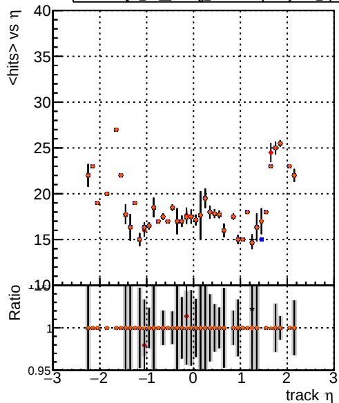
Legend: — DQM_TT original (blue line with dots) — DQM_TT debug_bestinlayer75_epcoh10 (red line with dots) — DQM_TT debug_truthallhits75_epcoh11 (black line with dots) — DQM_TT debug_truthsimuptolayer75_epcoh11 (orange line with dots)
