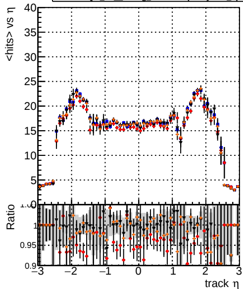
Legend: DQM_TT original (blue line), DQM_TT debug_bestinlayer75_epcoh10 (red line), DQM_TT debug_truthallhits75_epcoh11 (black line), DQM_TT debug_truthsimuptolayer75_epcoh11 (orange line). mean hits
