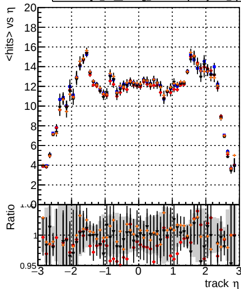
Legend: DQM_TT original (blue line), DQM_TT debug_bestinlayer75_epcoh10 (red line), DQM_TT debug_truthallhits75_epcoh11 (black line), DQM_TT debug_truthsimuptolayer75_epcoh11 (orange line) mean hits
