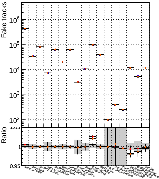
Number Symbol Label —▲— DQM_TT_paretofrontMinFROnlyFWD2_PU —+— DQM_TT_paretofrontMaxHitsOnlyFWD2_PU
