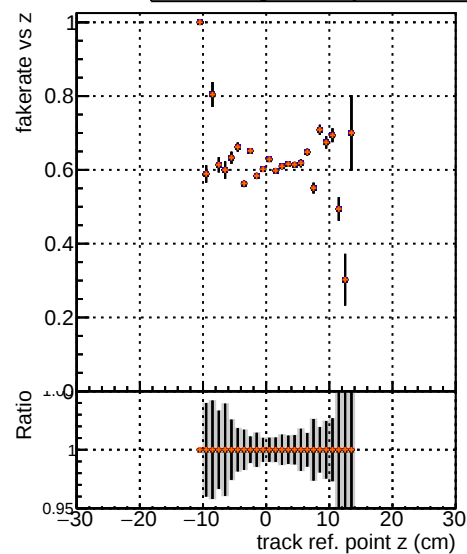
Fake rate vs verpos Legend: DOM TT original noPU DOM TT paretofrontMaxEffOnlyFWD2_PU DOM TT paretofrontMinHitOnlyFWD2_PU DOM TT paretofrontMaxHitOnlyFWD2_PU
