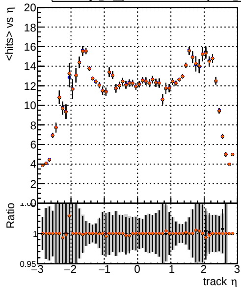
mean hits DQM_TT original_noPU DQM_TT paretofrontMaxEffOnlyFWD2_PU DQM_TT paretofrontMinFOnlyFWD2_PU DQM_TT paretofrontMaxHitsOnlyFWD2_PU
