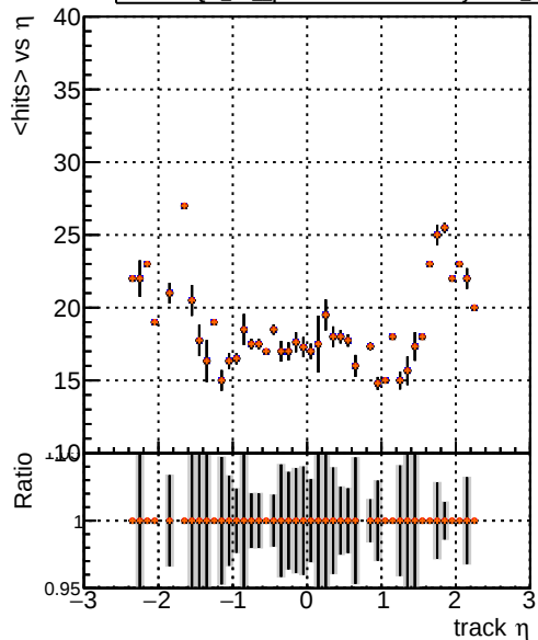
mean hits DQM_TT original noPU DQM_TT paretofrontMaxEffOnlyFWD2_PU DQM_TT paretofrontMinFWD2_PU DQM_TT paretofrontMaxHitsOnlyFWD2_PU
