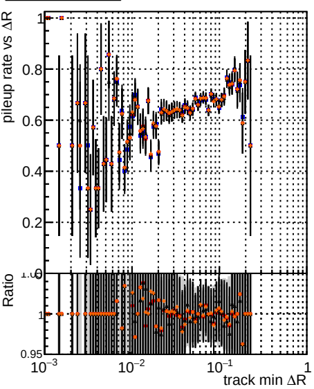
Fake rate vs \Delta R (track, jet) | Duplicates Rate vs \Delta R (track, jet) | Pileup rate vs \Delta R (track, jet) Legend: original noPU paretofrontMinEffOnlyFWD2_PU paretofrontMinHitOnlyFWD2_PU paretofrontMaxHitOnlyFWD2_PU
