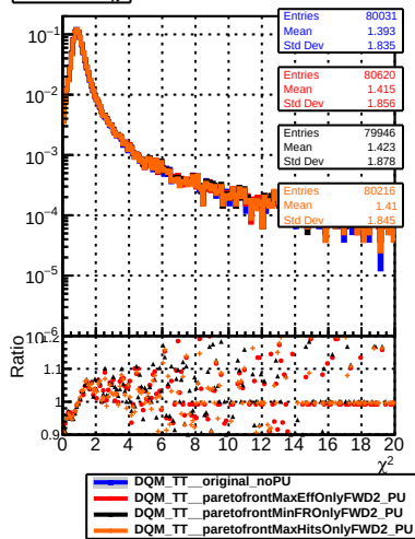
normalized \chi^2
