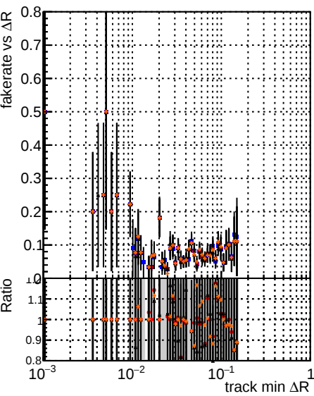
Fake rate vs \Delta R(\text{track, jet}) Legend: original noPU paretofrontMaxEffOnlyFWD2_PU paretofrontMinHitOnlyFWD2_PU paretofrontMaxHitOnlyFWD2_PU
