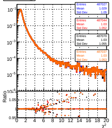
normalized \chi^2
