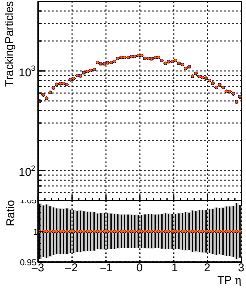
N of simulated tracks vs \eta —•— DQM TT original_noPU —•— DQM TT paretofrontMaxEffOnlyFWD2_PU —•— DQM TT paretofrontMinFROOnlyFWD2_PU —•— DQM TT paretofrontMaxHitsOnlyFWD2_PU
