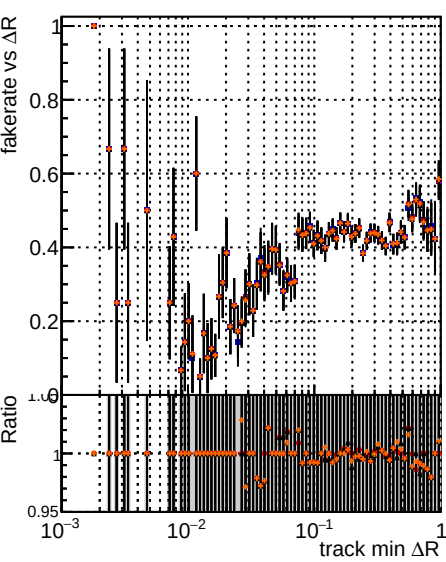
Fake rate vs \Delta R(\text{track, jet}) | Duplicates Rate vs \Delta R(\text{track, jet}) | Pileup rate vs \Delta R(\text{track, jet}) Legend: original noPU paretofrontMaxEffOnlyFWD2_PU paretofrontMinHitOnlyFWD2_PU paretofrontMaxHitOnlyFWD2_PU
