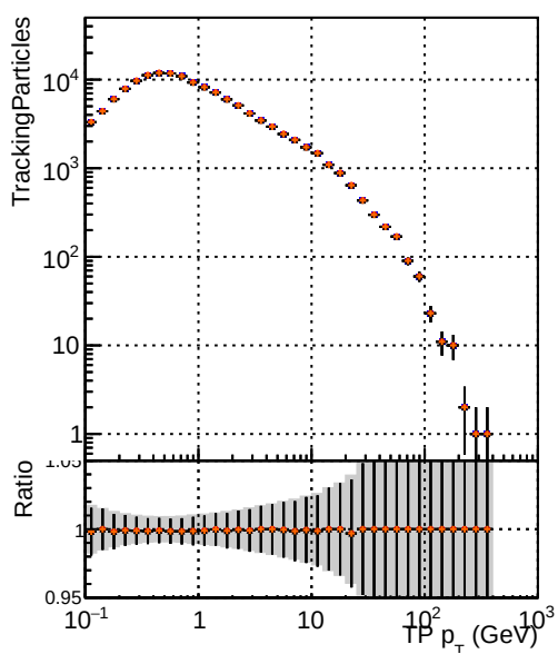
N of simulated tracks vs TP p_T
