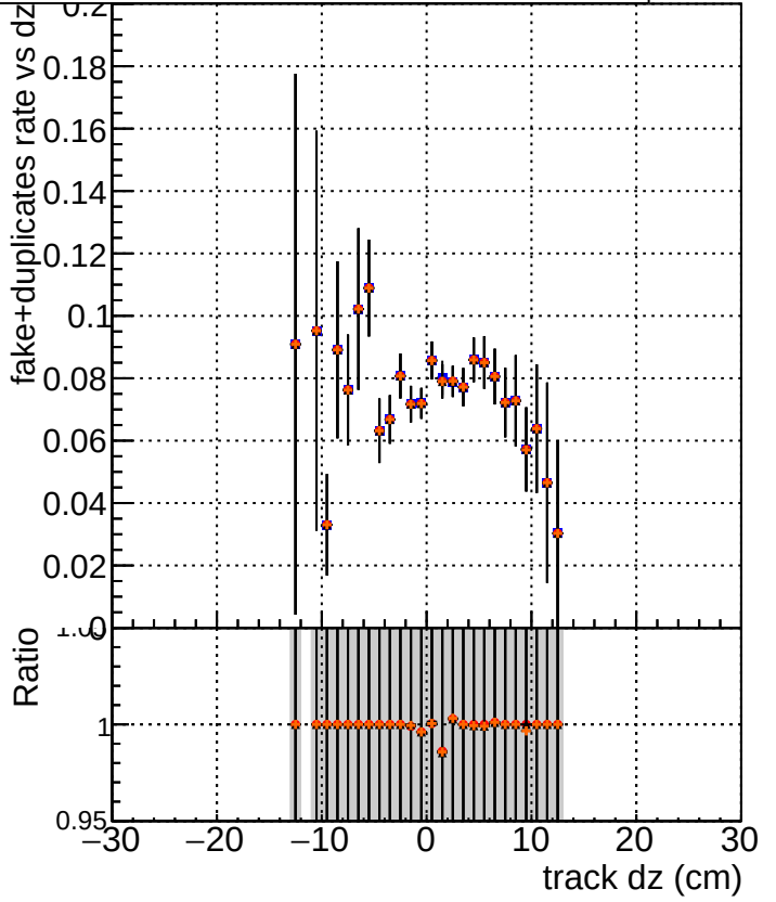
DQM_TT_original_noPU DQM_TT_paretofrontMaxEffOnlyFWD2_PU DQM_TT_paretofrontMinFROnlyFWD2_PU DQM_TT_paretofrontMaxHitsOnlyFWD2_PU
