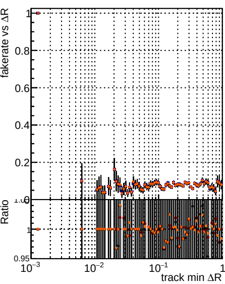
Fake rate vs \Delta R(\text{track, jet}) Legend: original noPU paretofrontMaxHitOnlyFWD2_PU paretofrontMinHitOnlyFWD2_PU paretofrontMaxHitOnlyFWD2_PU
