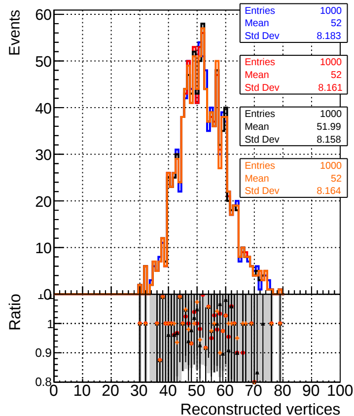
Reconstructed Vertices in Event
