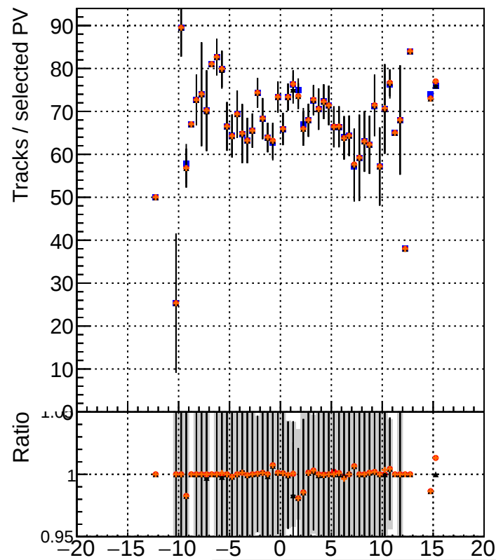
Reconstructed Tracks in Vertex (tagged Vtx) vs Z
