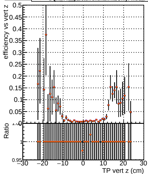
Efficiency vs. TP vert z (cm) —●— DQM_TT original_noPU —●— DQM_TT paretofrontMaxEffOnlyFWD2_PU —●— DQM_TT paretofrontMinFROnlyFWD2_PU —●— DQM_TT paretofrontMaxHitsOnlyFWD2_PU
