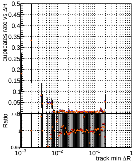
Legend for Fake rate vs \Delta R , Duplicates Rate vs \Delta R , and Pileup rate vs \Delta R : - \Delta R (black line with dots): original noPU - \Delta R (red line with dots): paretofrontMaxEffOnlyFWD2_PU - \Delta R (blue line with dots): paretofrontMinHitOnlyFWD2_PU - \Delta R (orange line with dots): paretofrontMaxHitOnlyFWD2_PU
